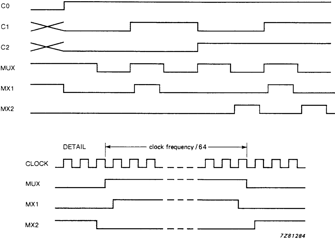
Fig.4 Timing diagram.
