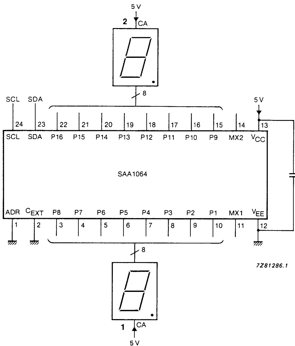
Fig.6 Static mode application diagram.
