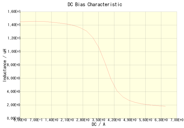
SLF10145T-150M2R2-PF(Amb. Temp. = 20degc)
