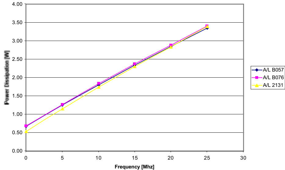
Edge 818AHF Power Dissipation vs. Frequency
