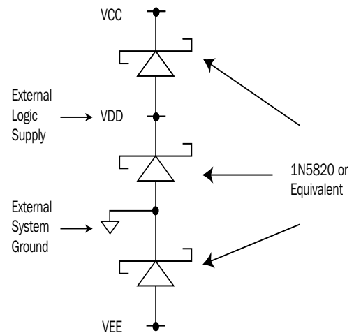
Figure 3. Power Supply Protection Scheme
