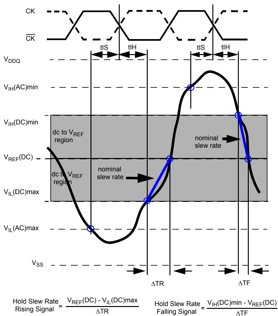
Figure 17. Illustration of nominal slew rate for tlH
