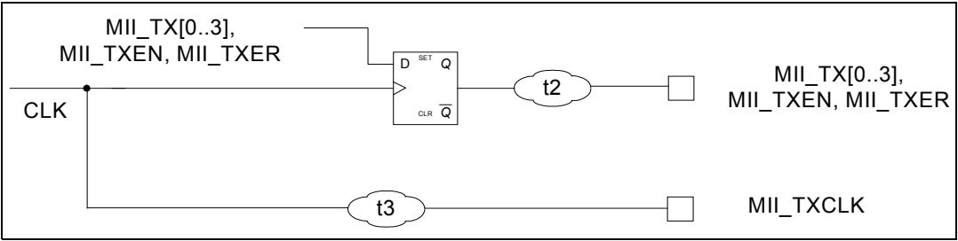
Figure 29. Block diagram of MII TX pins
